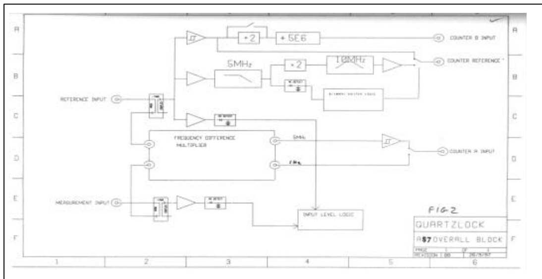
Fig 1 Overall block diagram
