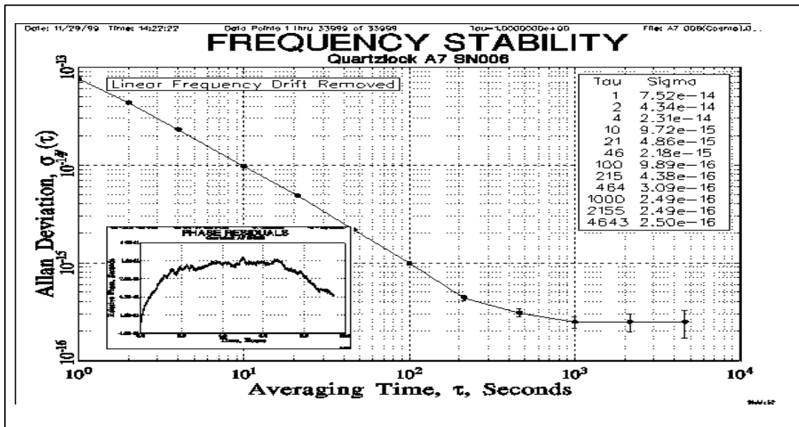
Fig 5 Allan Variance Noise Floor
